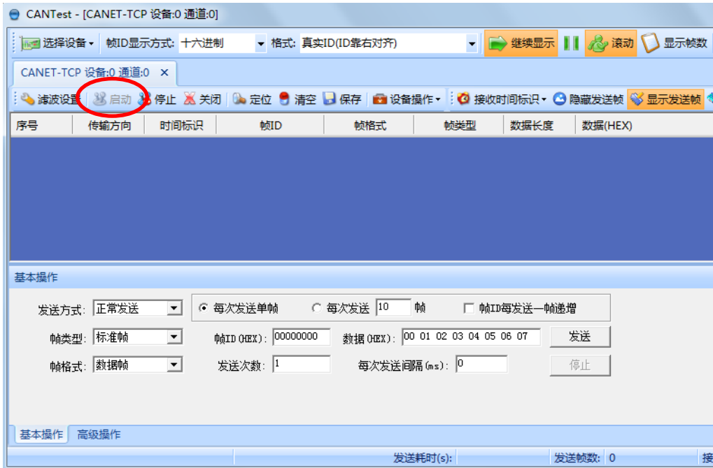
图 4.14 启动 CANET-100T/200T
